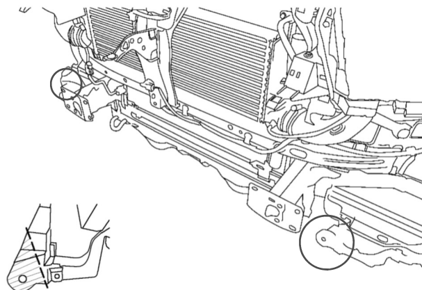
Fender Liner - Lower RHS shown
