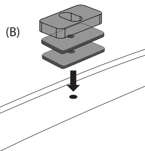
The spacer will sit above the 2x butyl patches
