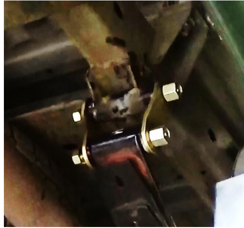
Figure 4: After greasable shackle installation
