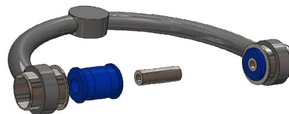
Figure 02 – Front upper Control Arm, bushing installation
