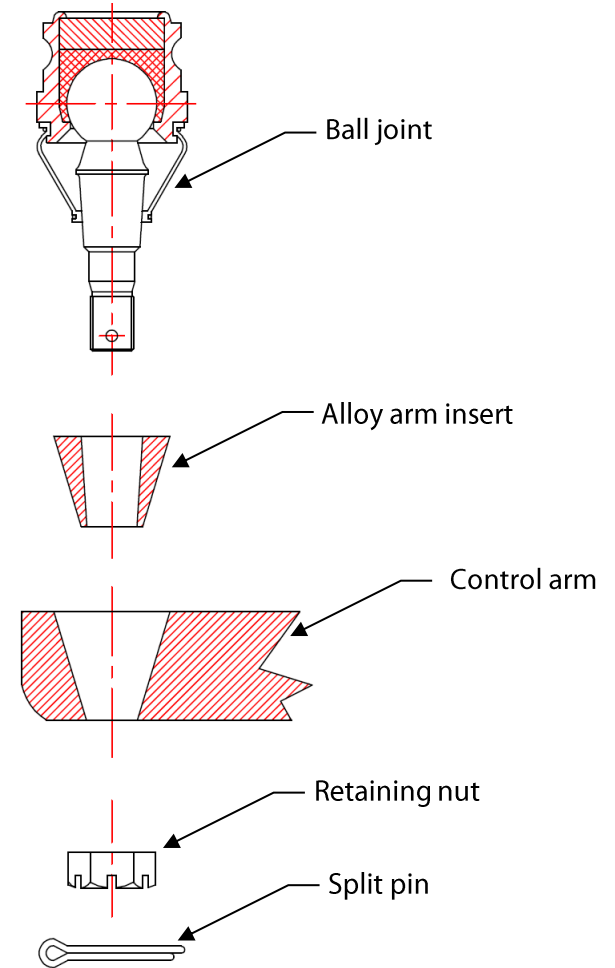
Figure 3: Roll center ball joint fitting schematic
