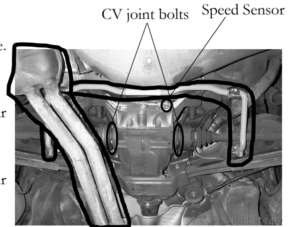
Figure 01 – Underside of Rear of Car with elements to remove highlighted.
