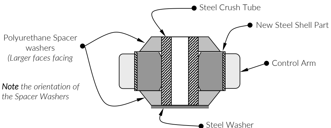
Figure 02 – Front Lower Control Arm Rear Bush Installation
