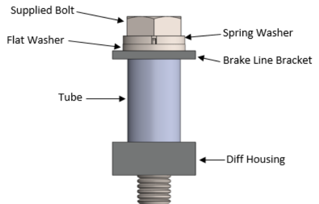
Picture 5: Assembly of brake hose mount spacer
