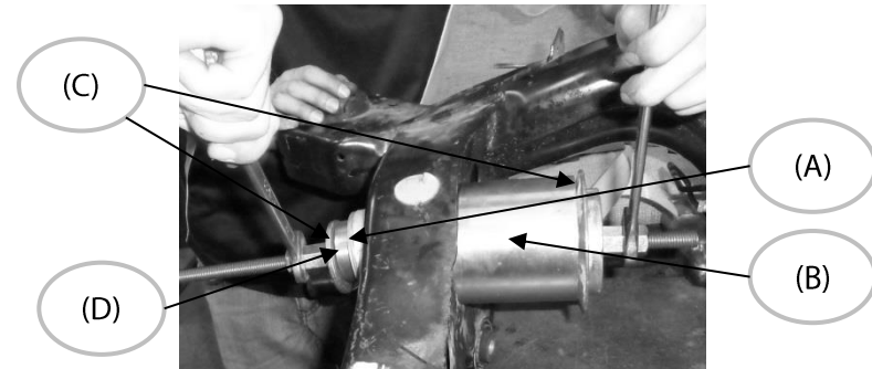
Tools setup for factory bushes removal
