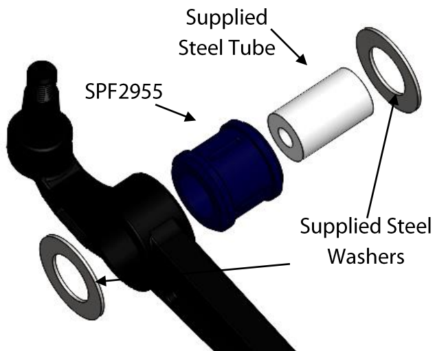
Figure 1: Bushing Orientation
