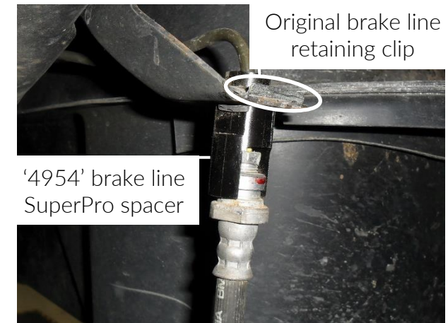
Figure 03 - Installed '4954' brake line spacer
