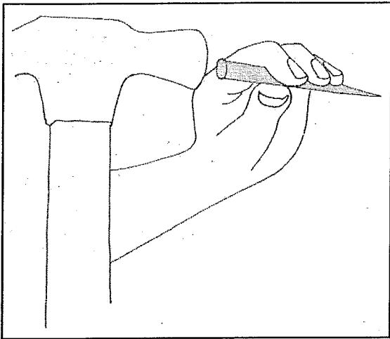
Diagram 7: Centre punch all marked locations.
