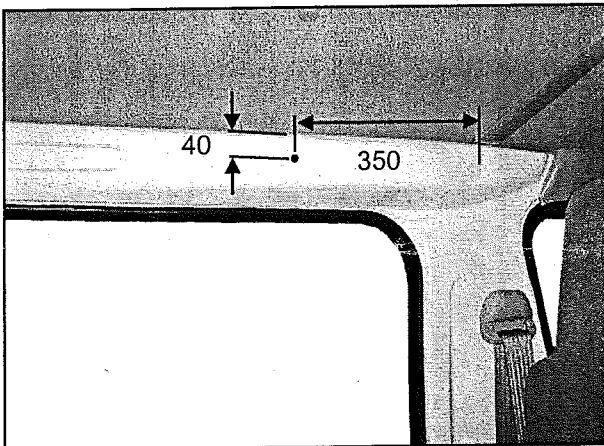
Diagram 2: Top passenger side mount location.
