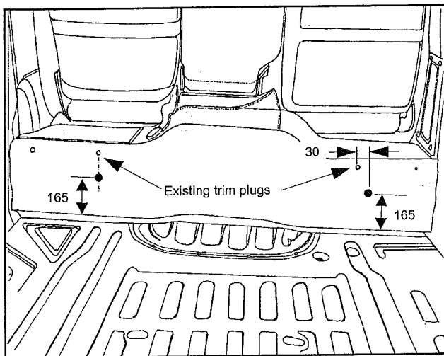
Diagram 3: Bottom mount locations in firewall.
