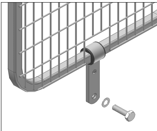
Diagram 21: Attaching bottom straps to vehicle.
