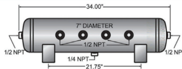
5 Gallon Air Tank Part # AC9051
