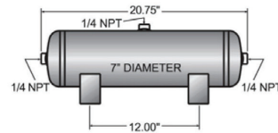
3 Gallon Air Tank Part # AC9031
