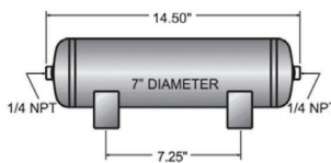
2 Gallon Air Tank Part # AC9020
