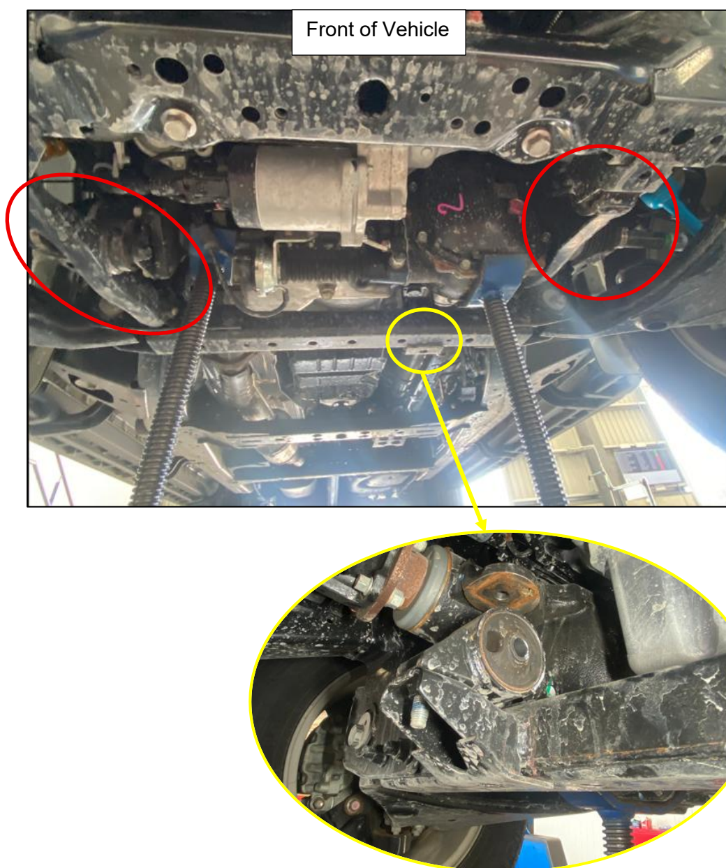
Figure 1: Differential Bracket Locations
